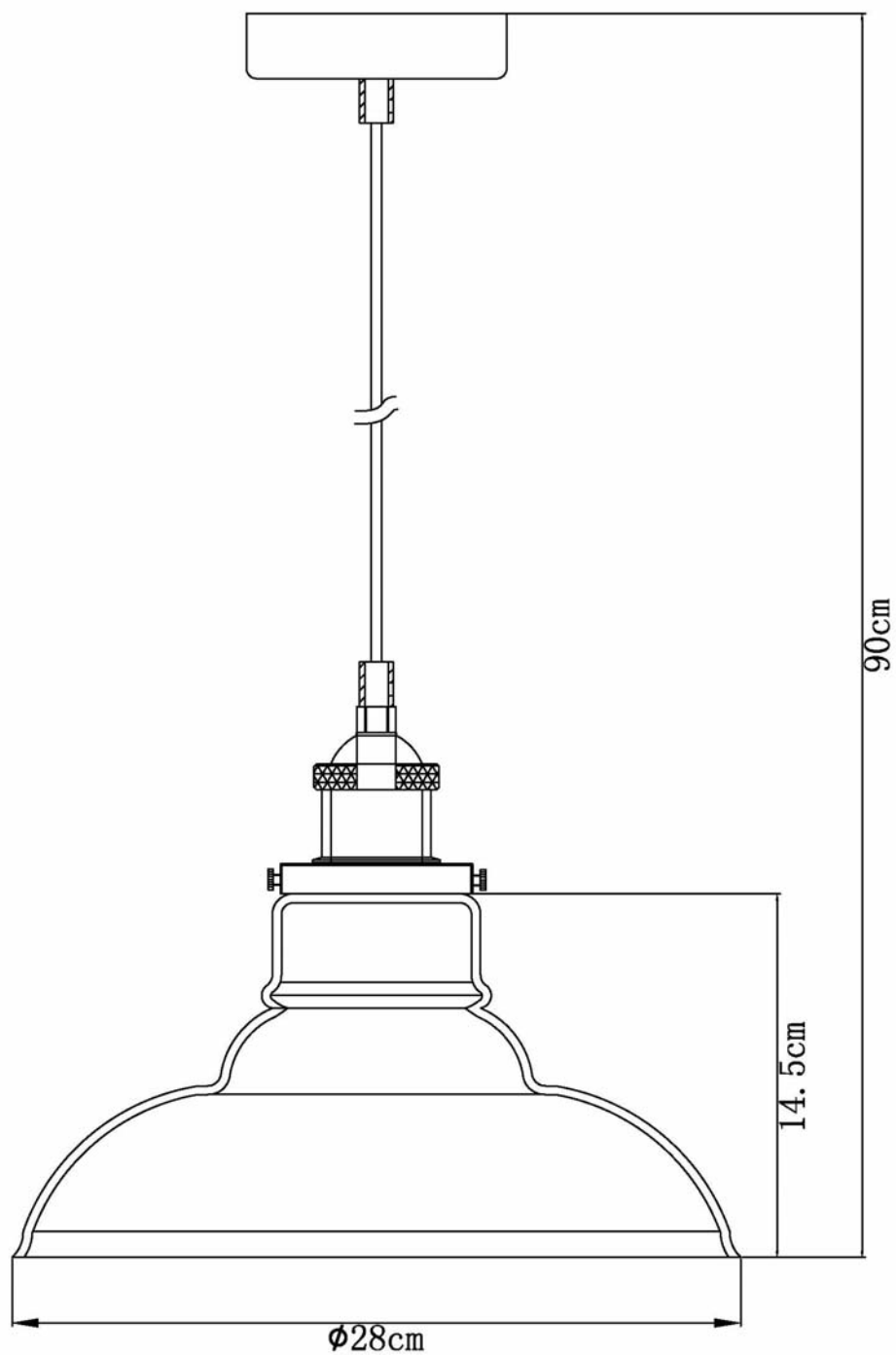
Line drawing of the item (with outline dimensions)
